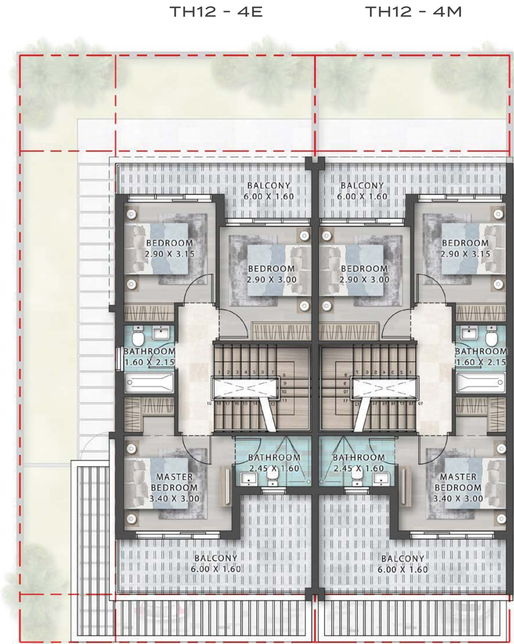
FIRST FLOOR
